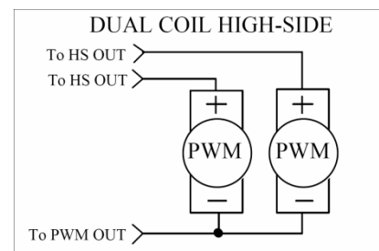
Connection detail showing connection for each output ( 1,2 and 3 ) channel
